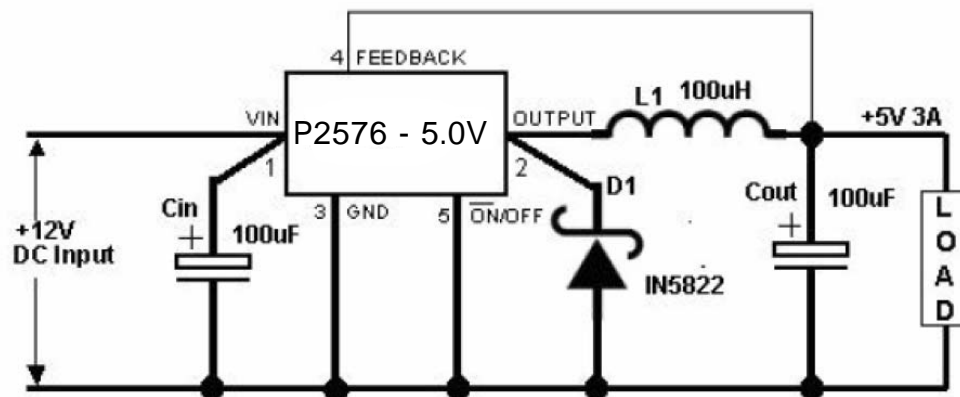
Figure 12. Typical Application of P2576 For 5V
