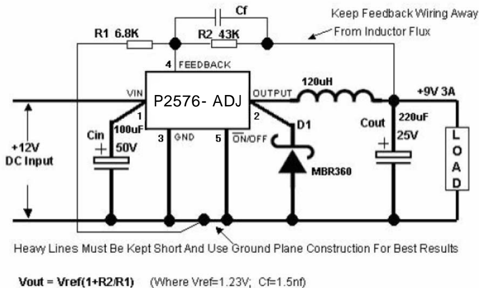
Figure 13. Typical Application of P2576 For ADJ
