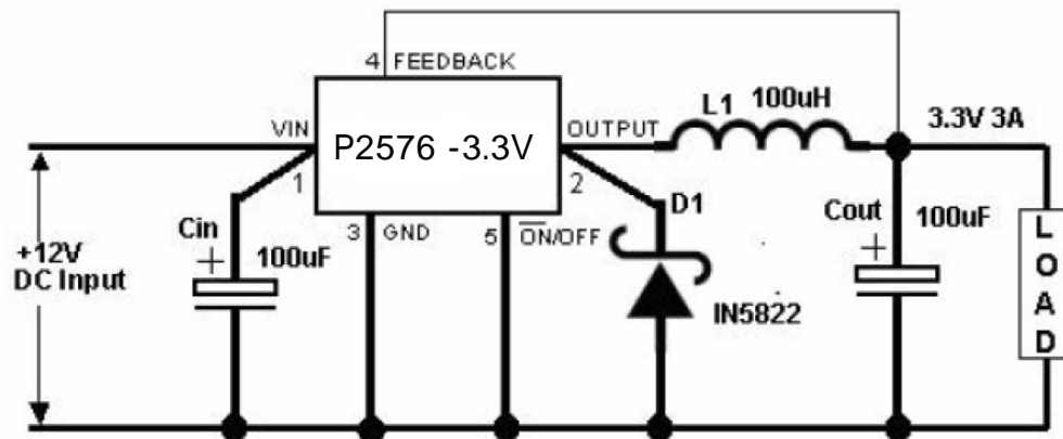
Figure 11. Typical Application of P2576 For 3.3V
