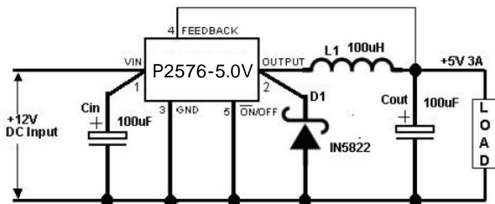
Figure 3. Typical Application of P2576
