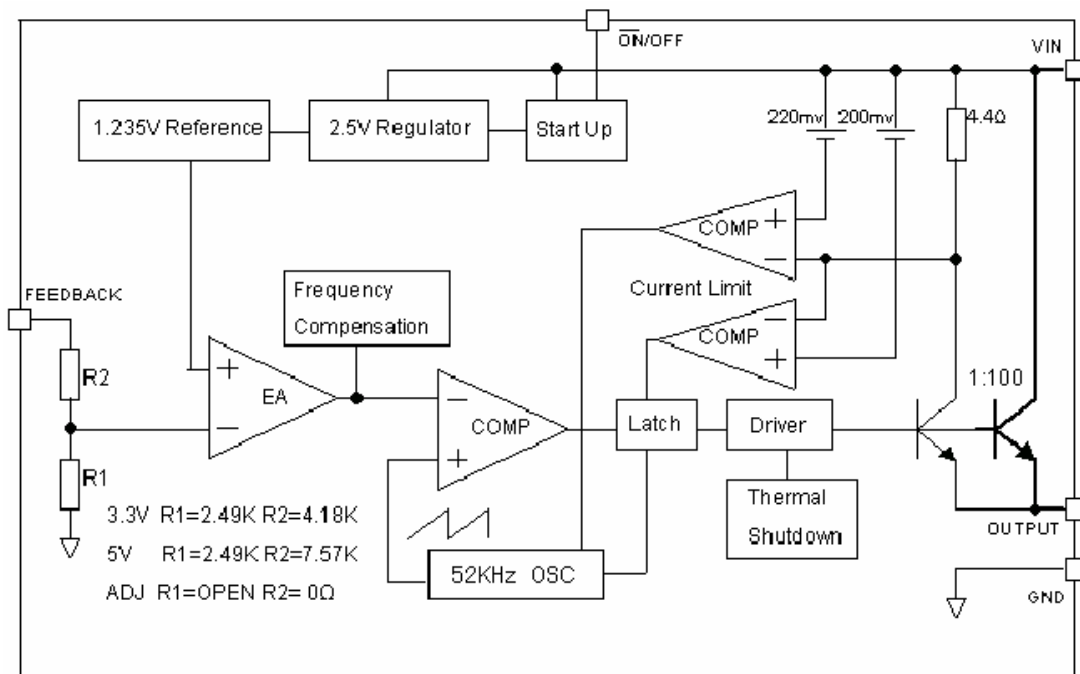
Figure 2. Functional Block Diagram of P2576
