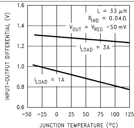
Figure 6. Dropout Voltage
