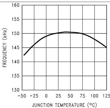
Figure 12. Switching Frequency
